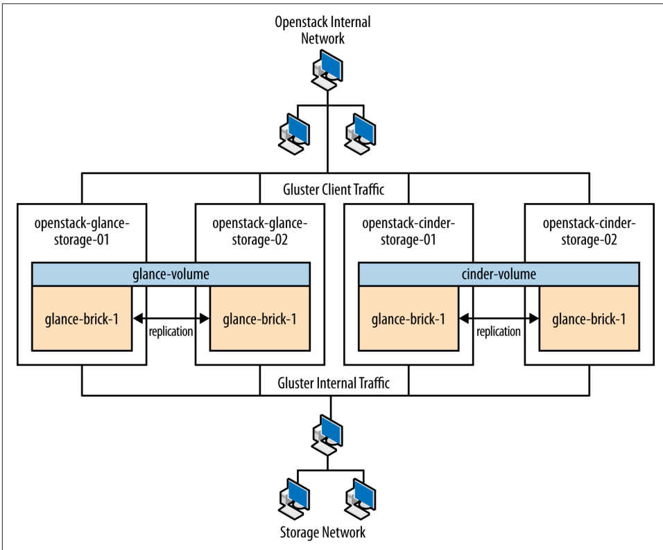
Figure 1-6. Storage node
