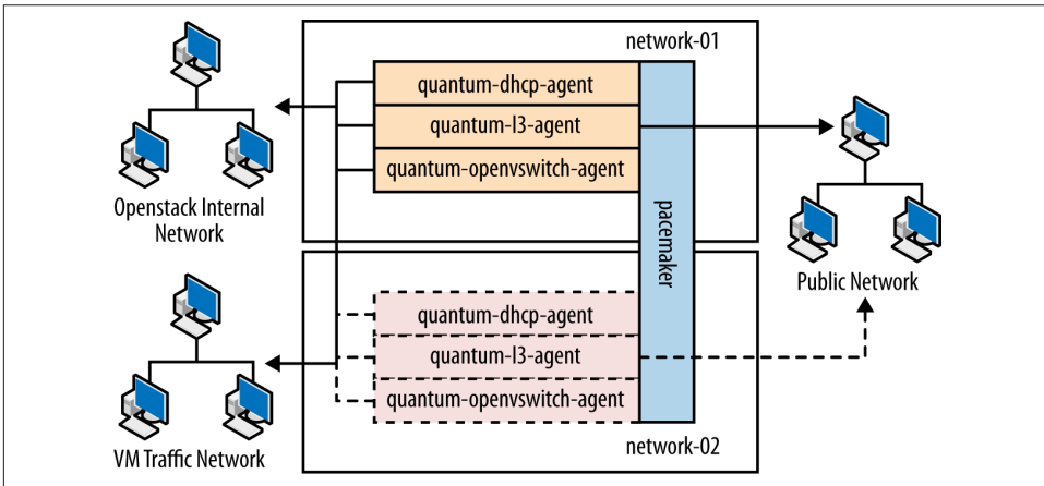
Figure 1-5. Network node
