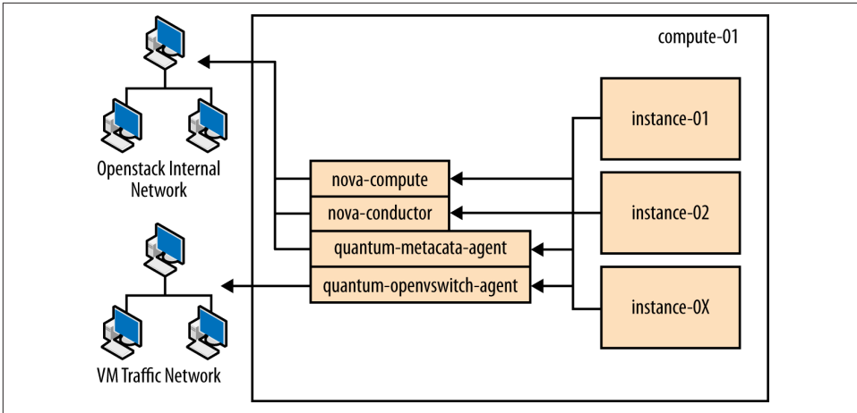
Figure 1-4. Compute node
